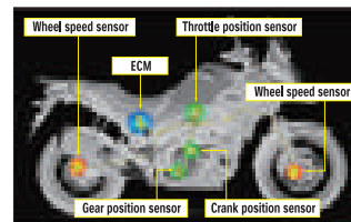
Advanced Traction Control System
